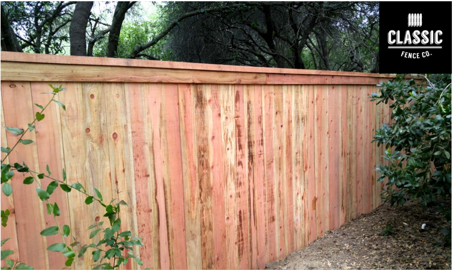
SOLID BOARD WITH CAP AND TRIM - BOARD SIDE
