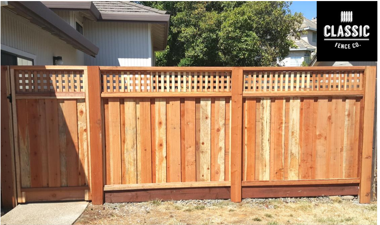
BOARD ON BOARD PICTURE FRAMED W/ SQUARE LATTICE & METAL POSTS
